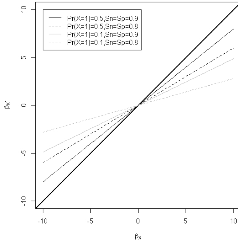
Figure 2: Effects of non-differential misclassification in binary X on the regression coefficient in a linear regression of continuous Y on X . \beta_X is the regression coefficient in a regression of Y on X and \beta_X^* is the regression coefficient in a regression of Y on X^* (misclassified X ). The attenuation factor \lambda (equation (13)) is a function of \Pr(X = 1) and the sensitivity ( Sn ) and specificity ( Sp ) of X^* . The thick line is the line \beta_X^* = \beta_X .
